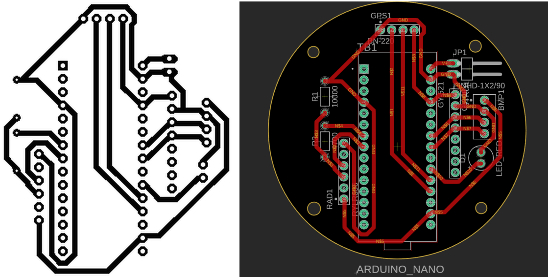
The PCB layout of the CanSat derived from the circuit schematic
